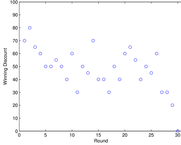
FIG 1. Winning Discount versus Rounds
